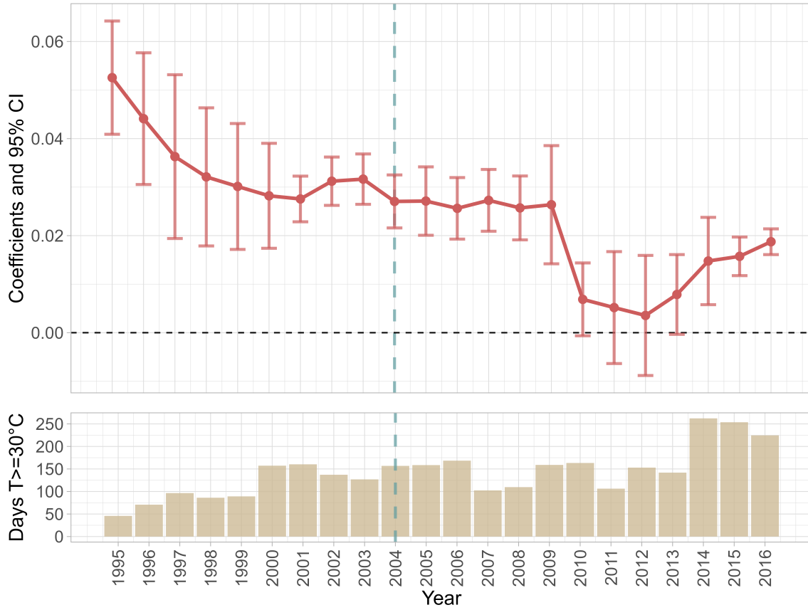
Figure 2: Trends in heat-related mortality across 7-year rolling samples
