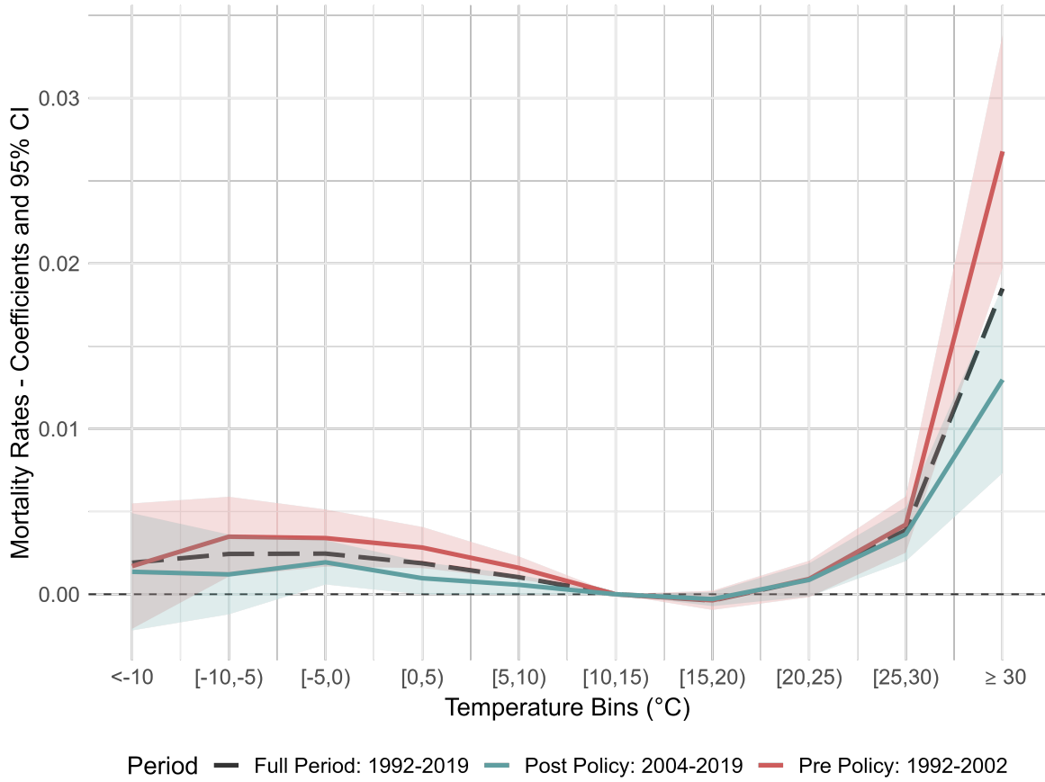
Figure 1: Temperature-mortality estimates for the pre- and post-policy periods
