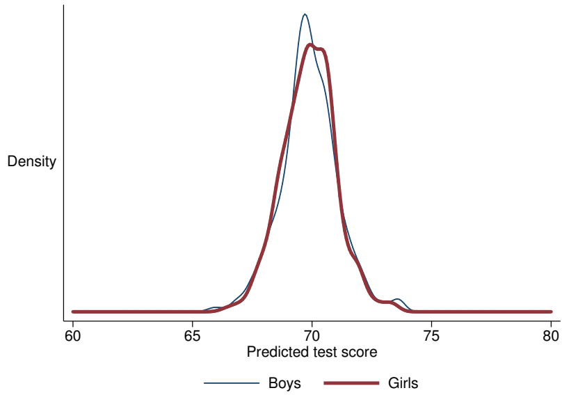
Figure A.1: Predicted test score distributions, by perceived ability
