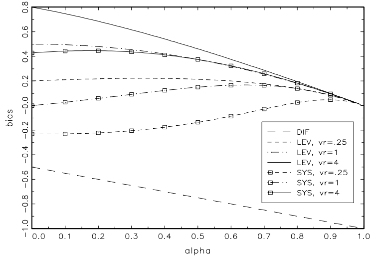
Figure 2. Asymptotic biases of OLS estimators, vr = \sigma_\eta^2/\sigma_v^2 = \{\frac{1}{4}, 1, 4\} .
