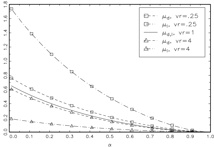
Figure 1. E\left(\frac{1}{N}\mu\right) as a function of \alpha , t = 6 and vr = \frac{\sigma_\eta^2}{\sigma_v^2} = \left\{\frac{1}{4}, 1, 4\right\} .
